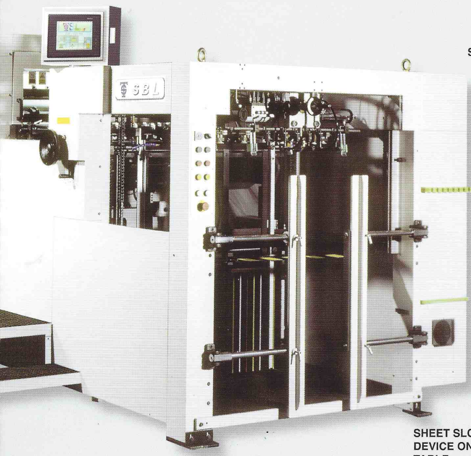
PAPER FEEDER
